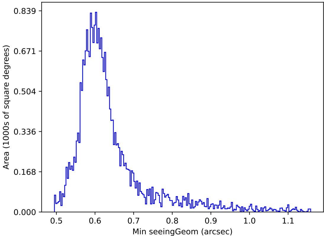
too_elab_r16_d2_griz_v3.4_10yrs Yr 1 i band: Min seeingGeom
