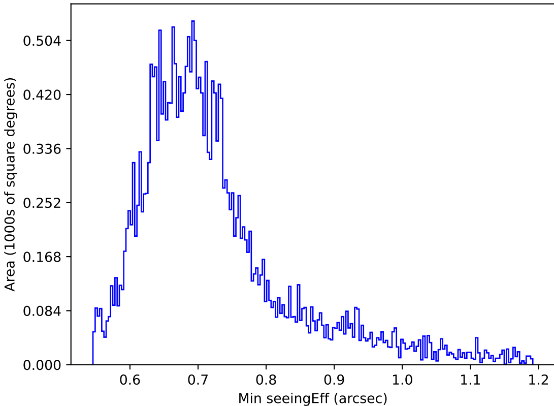
too_elab_r16_d2_griz_v3.4_10yrs Yr 1 z band: Min seeingEff
