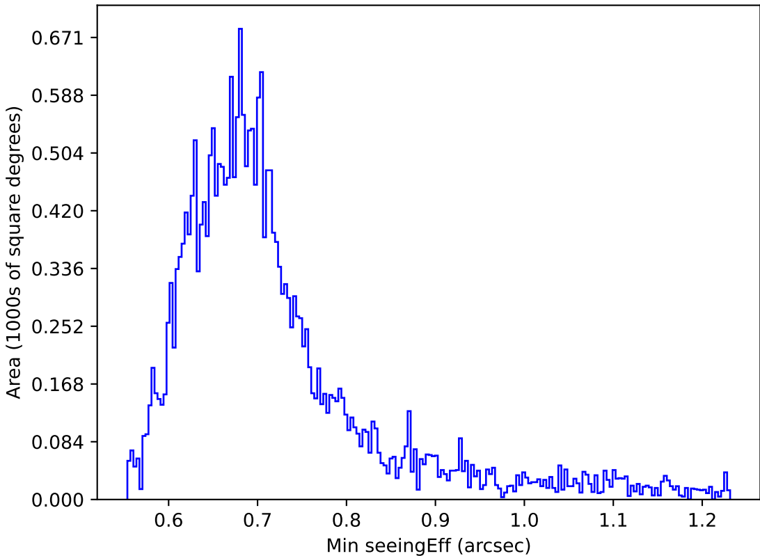
too_elab_r16_d2_griz_v3.4_10yrs Yr 1 r band: Min seeingEff
