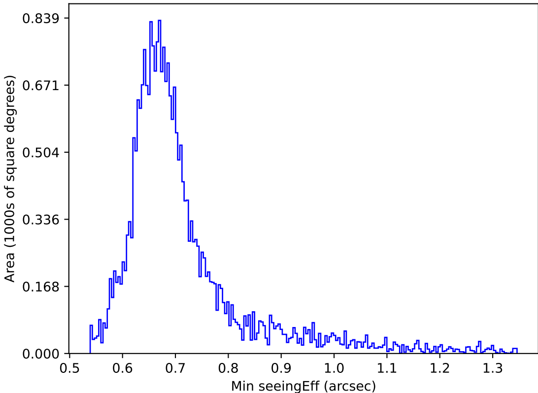
too_elab_r16_d2_griz_v3.4_10yrs Yr 1 i band: Min seeingEff
