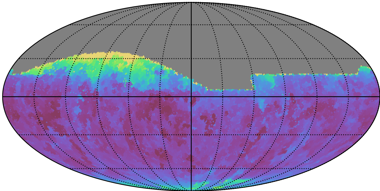
too_elab_r16_d2_griz_v3.4_10yrs Yr 1 all bands: Min seeingEff
