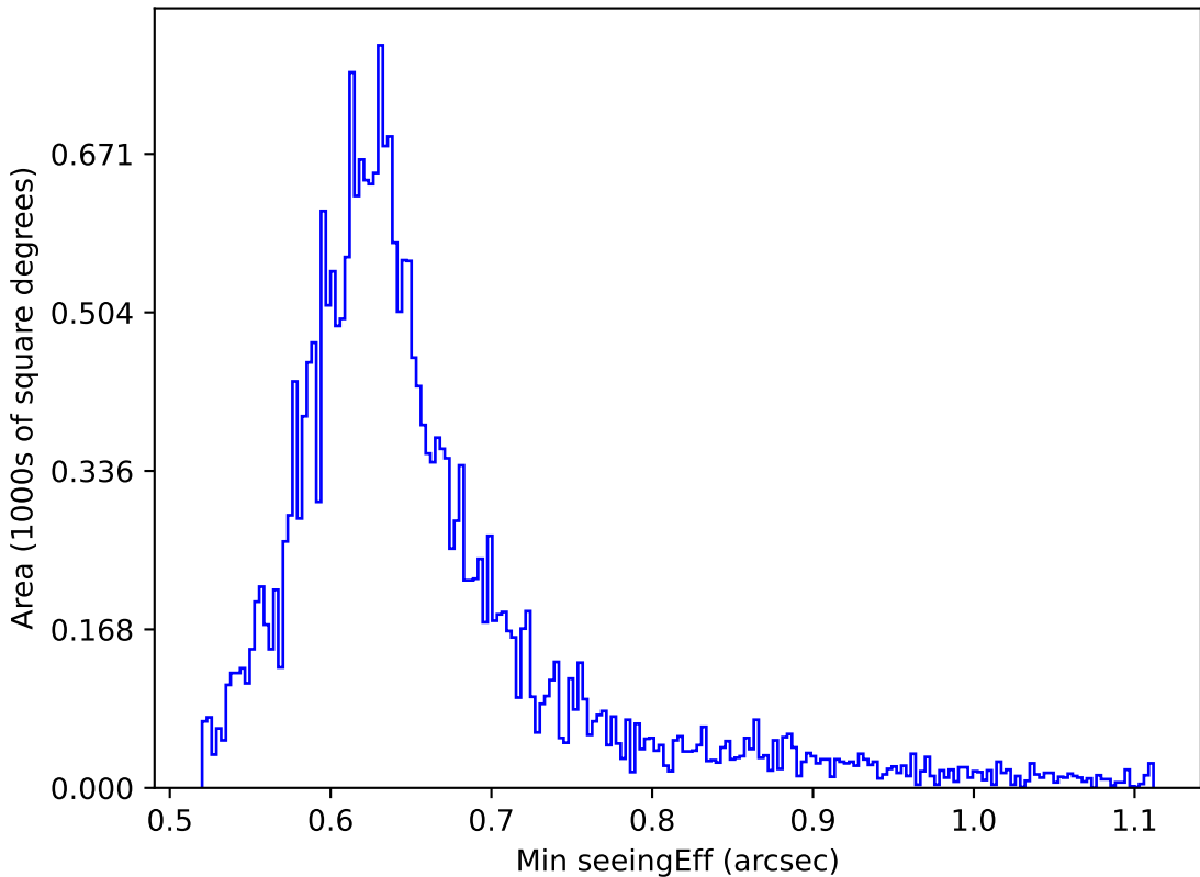
too_elab_r16_d2_griz_v3.4_10yrs Yr 1 all bands: Min seeingEff
