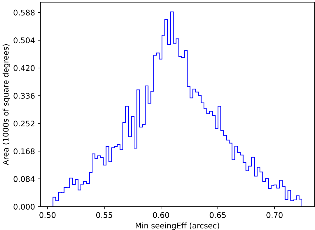
too_elab_r16_d2_griz_v3.4_10yrs WFD z band: Min seeingEff
