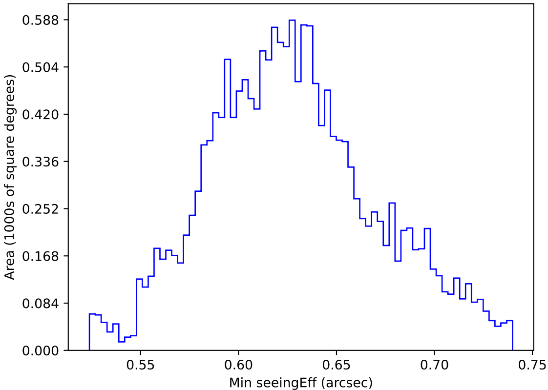
too_elab_r16_d2_griz_v3.4_10yrs WFD y band: Min seeingEff
