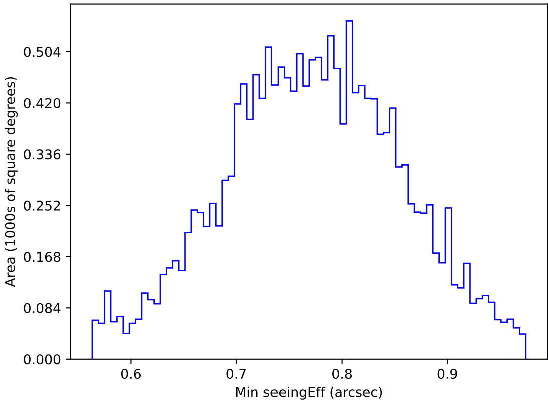
too_elab_r16_d2_griz_v3.4_10yrs WFD u band: Min seeingEff
