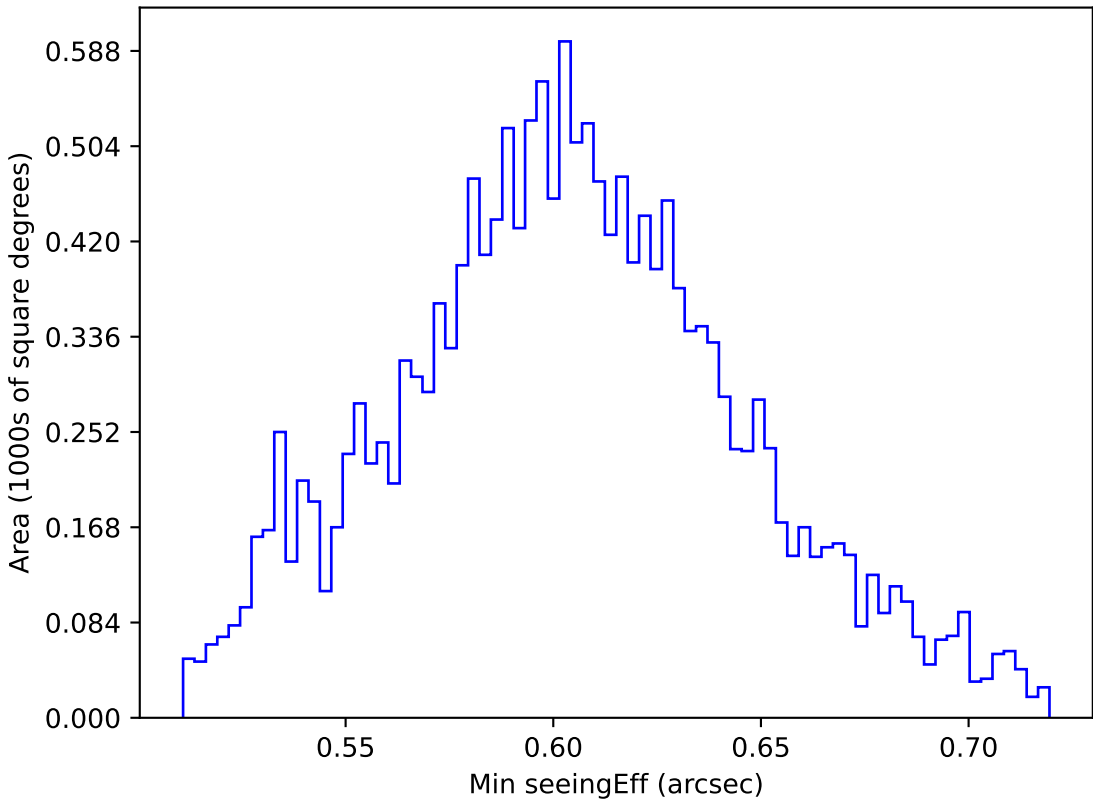
too_elab_r16_d2_griz_v3.4_10yrs WFD i band: Min seeingEff
