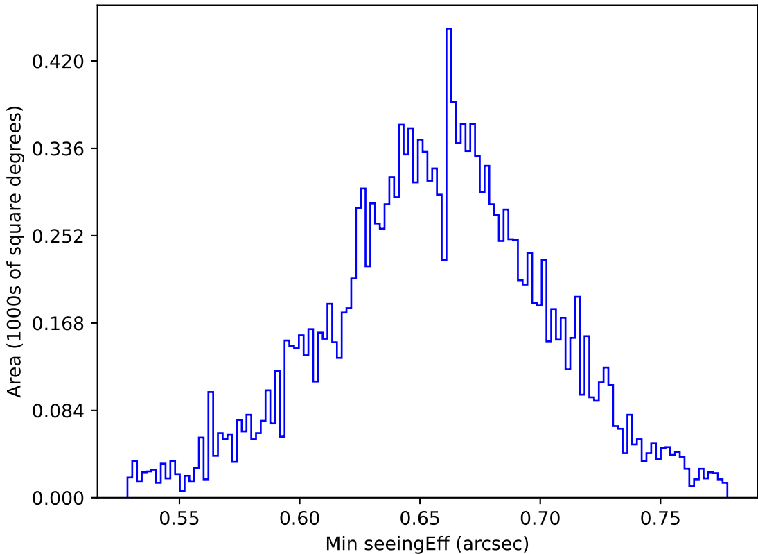
too_elab_r16_d2_griz_v3.4_10yrs WFD g band: Min seeingEff
