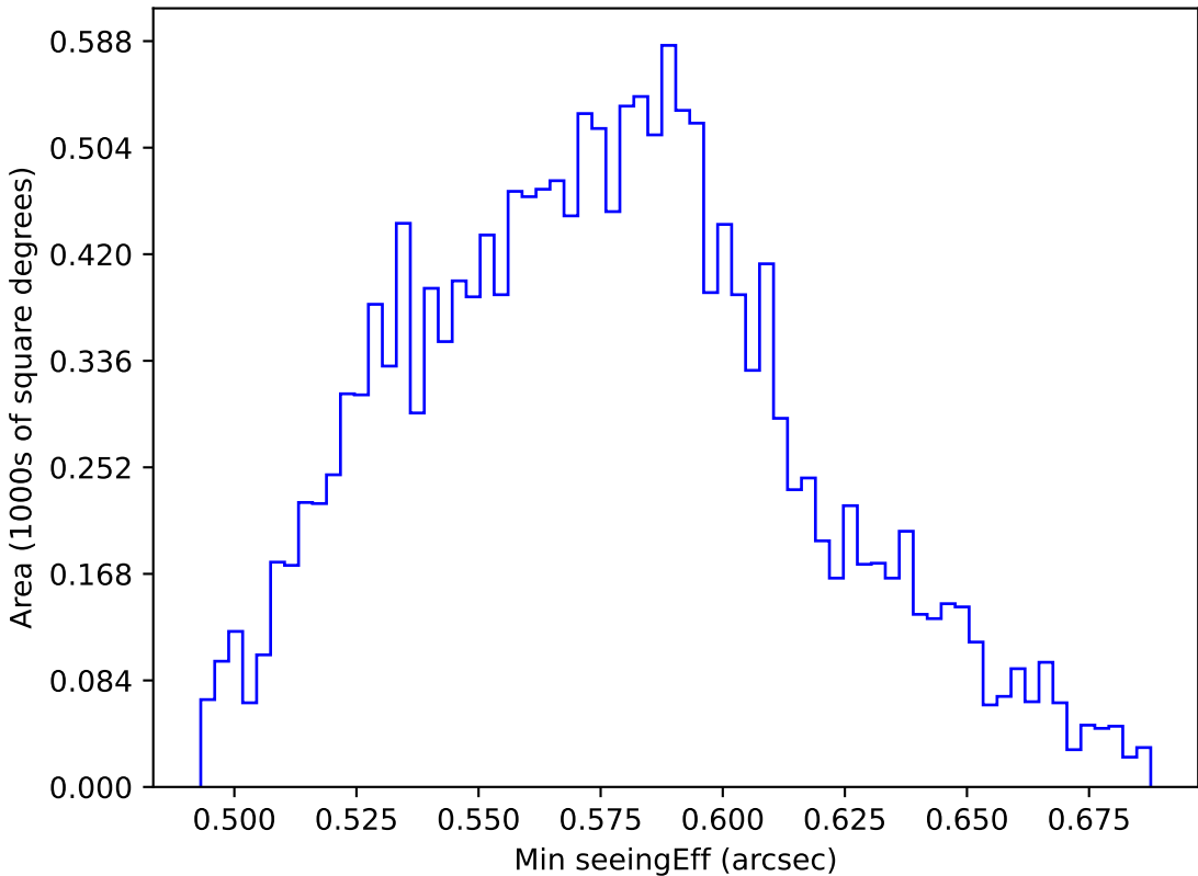
too_elab_r16_d2_griz_v3.4_10yrs WFD all bands: Min seeingEff
