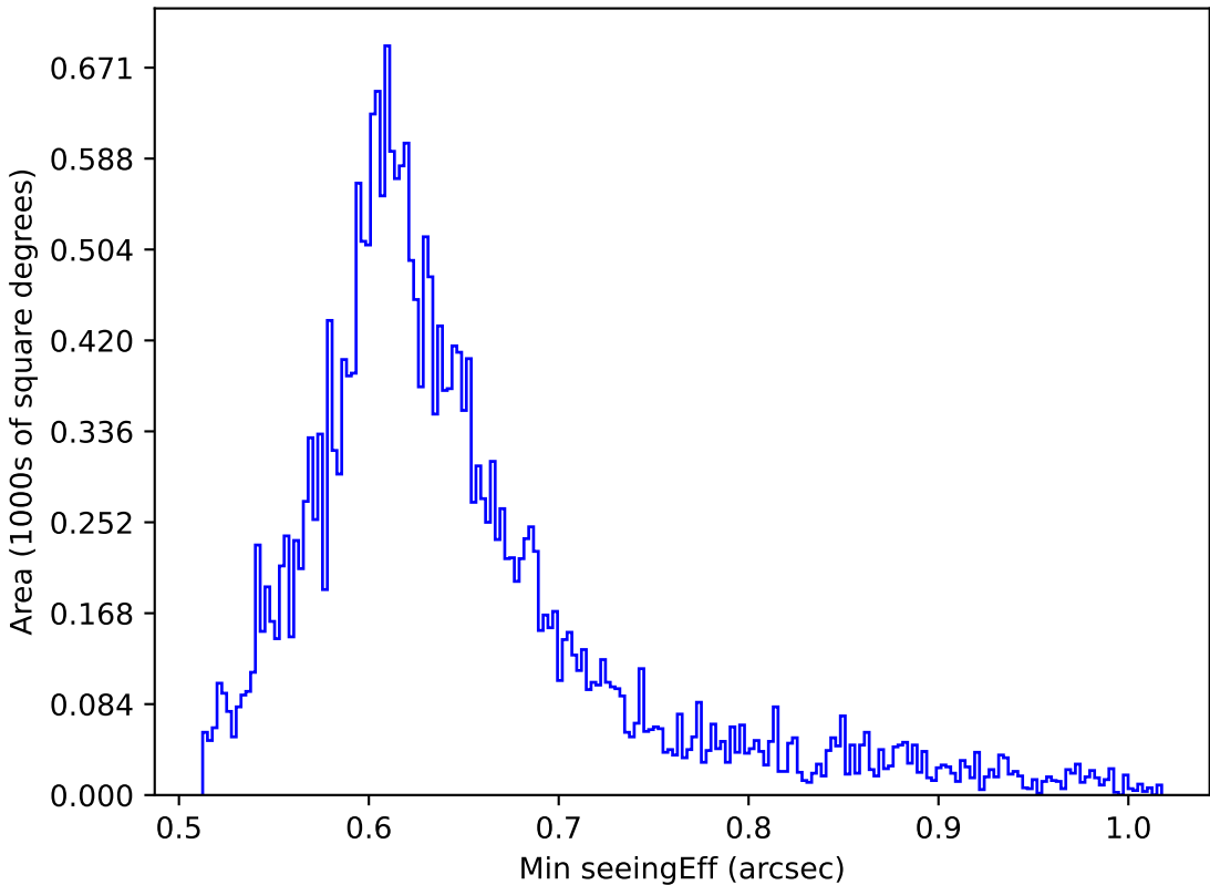
too_elab_r16_d2_griz_v3.4_10yrs All sky z band: Min seeingEff
