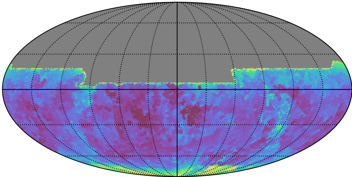
too_elab_r16_d2_griz_v3.4_10yrs All sky y band: Min seeingEff
