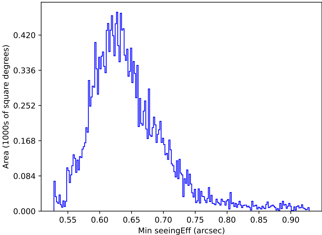
too_elab_r16_d2_griz_v3.4_10yrs All sky y band: Min seeingEff
