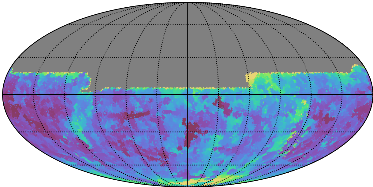
too_elab_r16_d2_griz_v3.4_10yrs All sky u band: Min seeingEff
