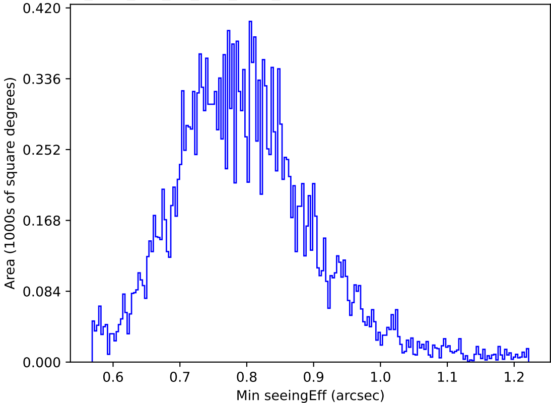
too_elab_r16_d2_griz_v3.4_10yrs All sky u band: Min seeingEff
