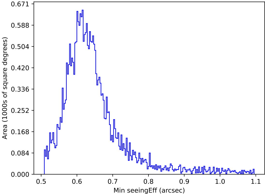
too_elab_r16_d2_griz_v3.4_10yrs All sky r band: Min seeingEff
