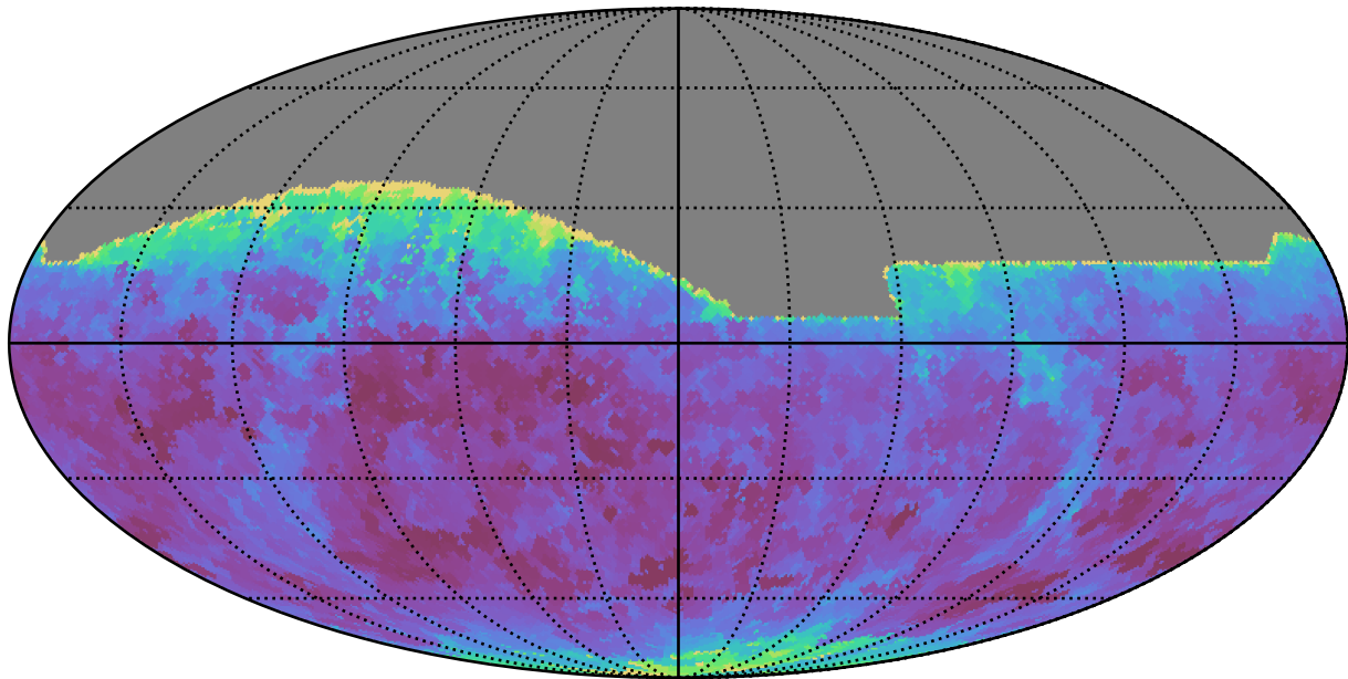
too_elab_r16_d2_griz_v3.4_10yrs All sky i band: Min seeingEff
