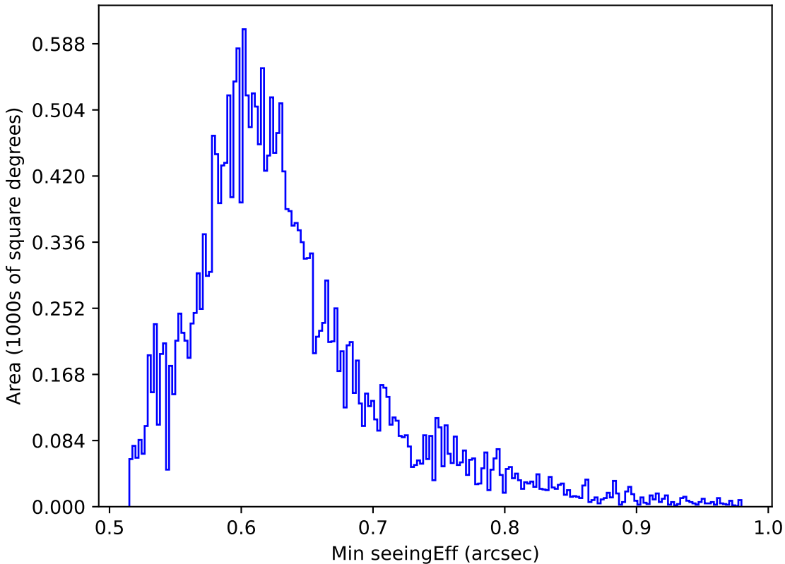
too_elab_r16_d2_griz_v3.4_10yrs All sky i band: Min seeingEff
