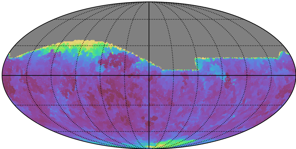
too_elab_r16_d2_griz_v3.4_10yrs All sky g band: Min seeingEff
