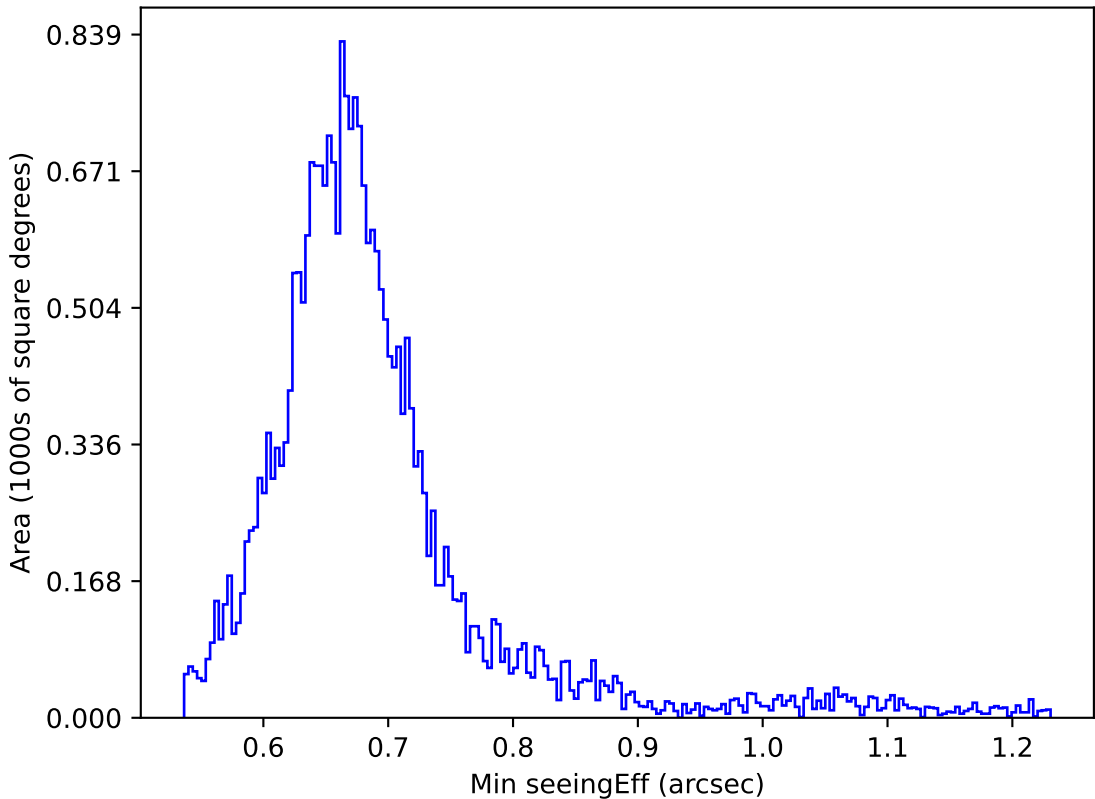
too_elab_r16_d2_griz_v3.4_10yrs All sky g band: Min seeingEff
