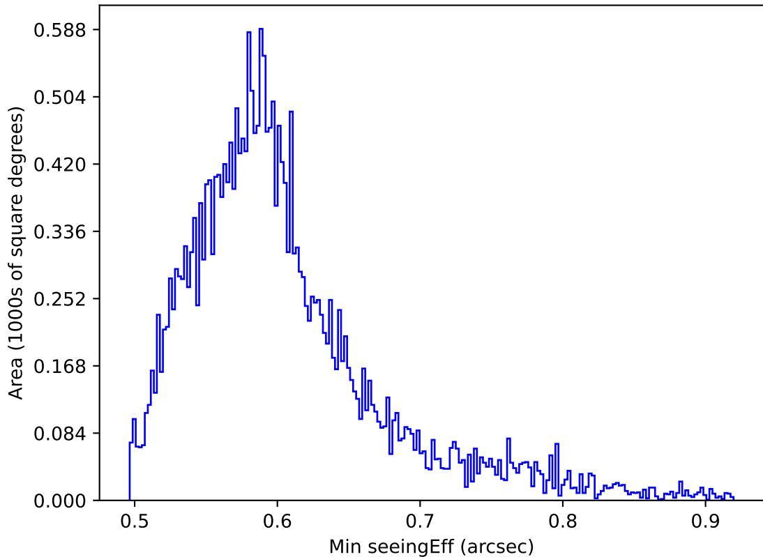
too_elab_r16_d2_griz_v3.4_10yrs All sky all bands: Min seeingEff
