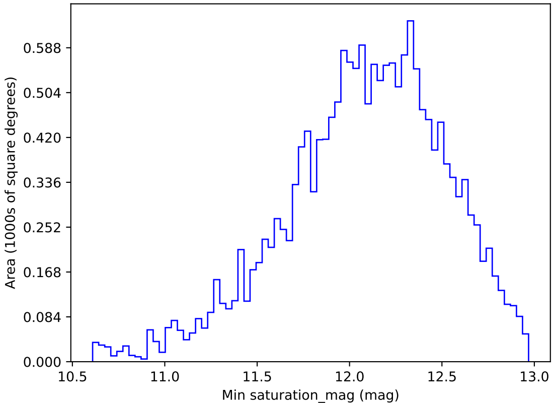
too_elab_r16_d2_griz_v3.4_10yrs WFD z band: Min saturation_mag
