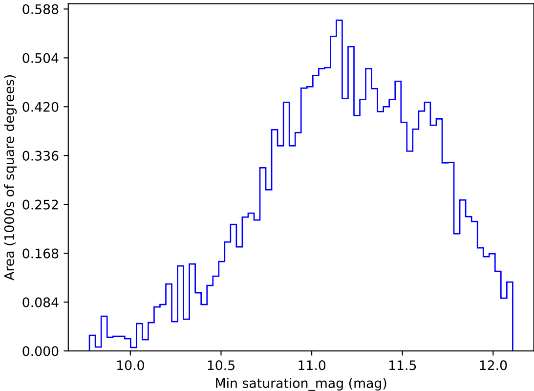
too_elab_r16_d2_griz_v3.4_10yrs WFD y band: Min saturation_mag
