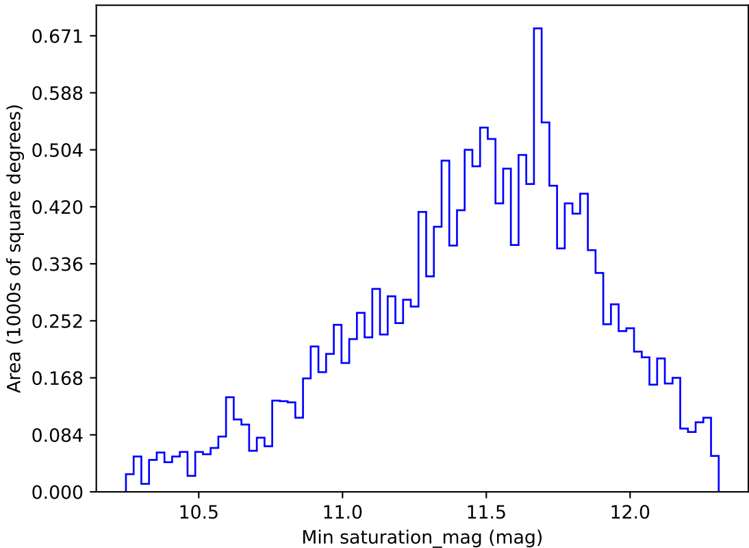
too_elab_r16_d2_griz_v3.4_10yrs WFD u band: Min saturation_mag
