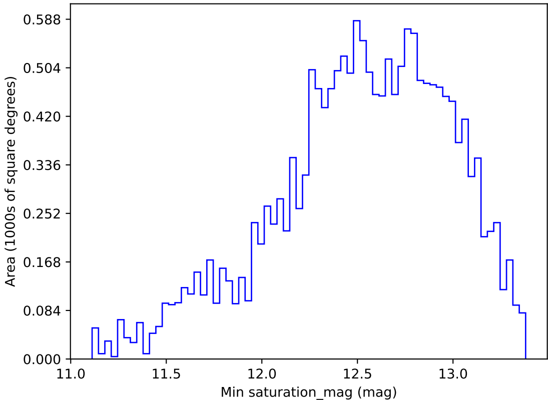
too_elab_r16_d2_griz_v3.4_10yrs WFD r band: Min saturation_mag
