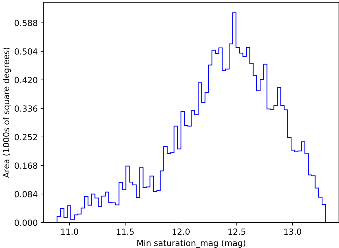
too_elab_r16_d2_griz_v3.4_10yrs WFD i band: Min saturation_mag
