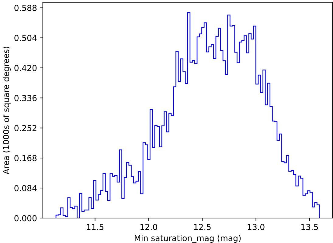
too_elab_r16_d2_griz_v3.4_10yrs All sky r band: Min saturation_mag
