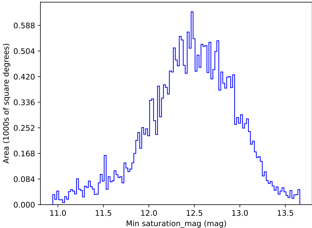
too_elab_r16_d2_griz_v3.4_10yrs All sky i band: Min saturation_mag
