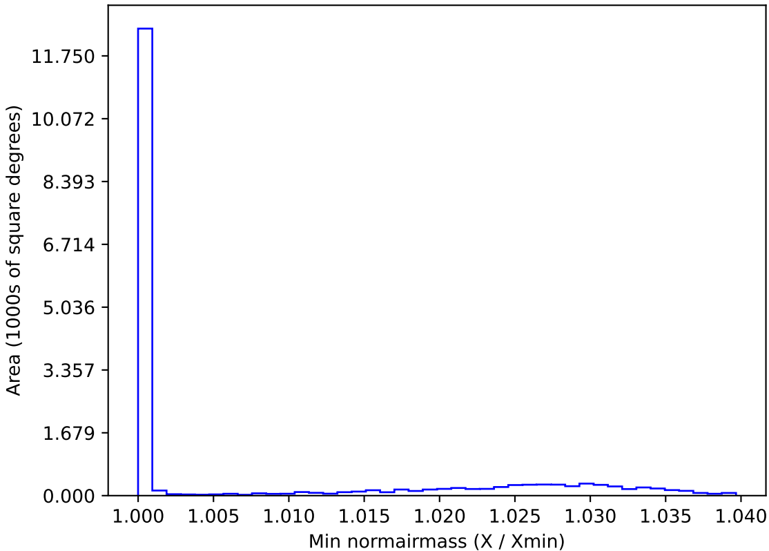
too_elab_r16_d2_griz_v3.4_10yrs WFD y band: Min normairmass
