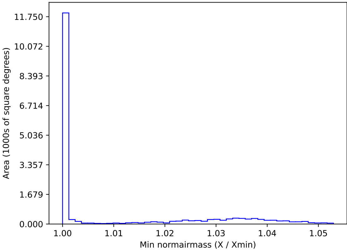
too_elab_r16_d2_griz_v3.4_10yrs WFD u band: Min normairmass
