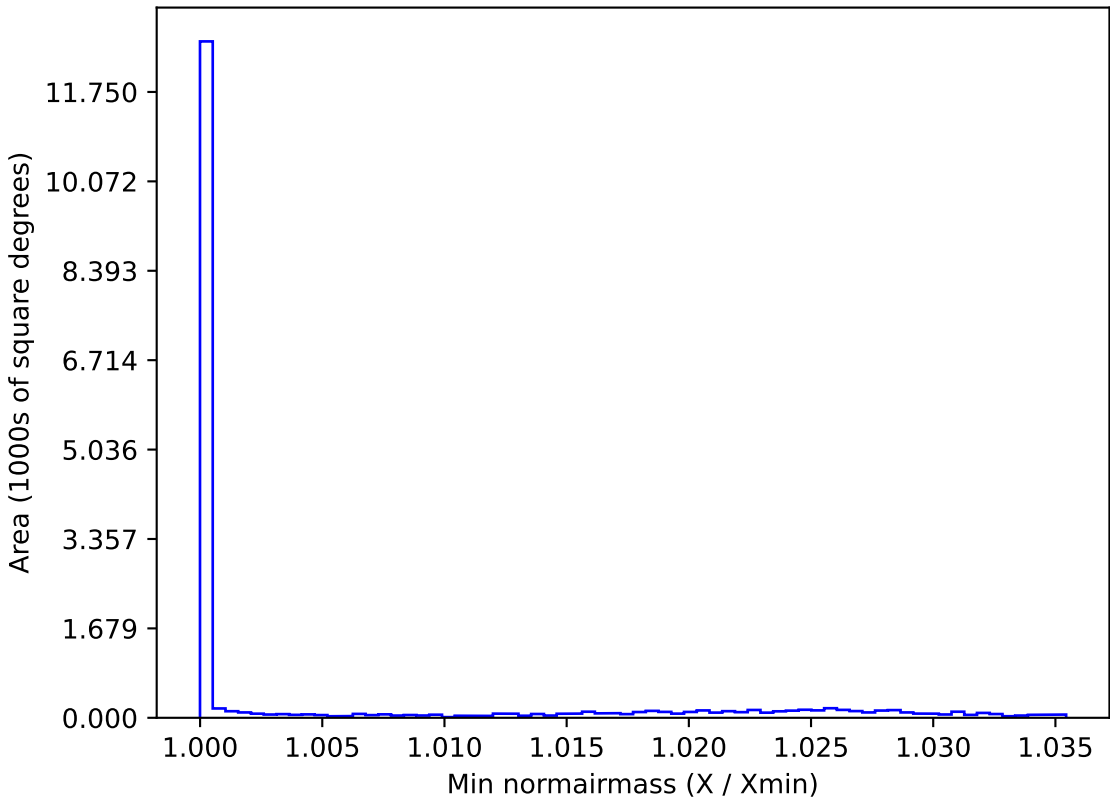
too_elab_r16_d2_griz_v3.4_10yrs WFD r band: Min normairmass
