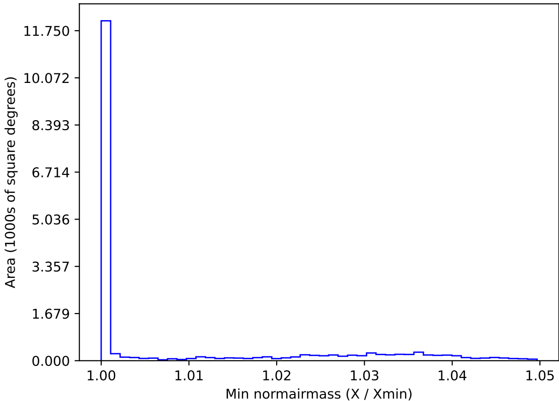
too_elab_r16_d2_griz_v3.4_10yrs WFD g band: Min normairmass
