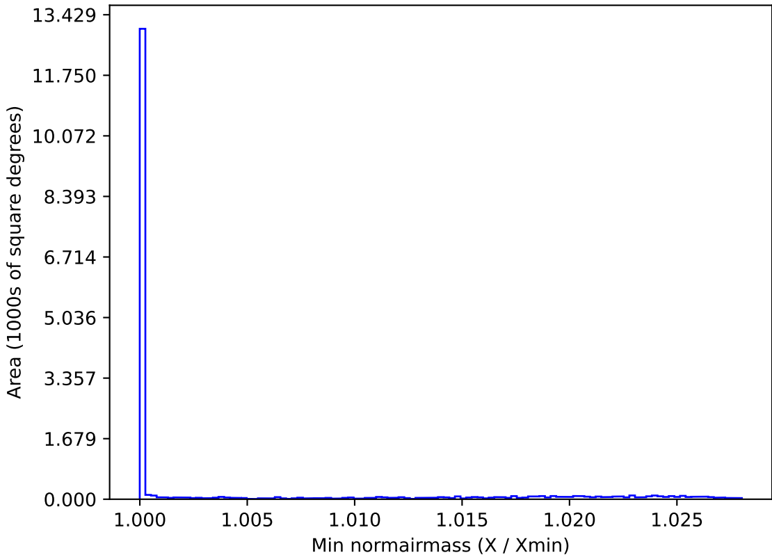
too_elab_r16_d2_griz_v3.4_10yrs WFD all bands: Min normairmass
