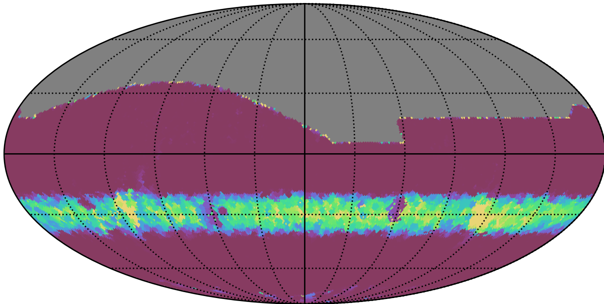
too_elab_r16_d2_griz_v3.4_10yrs All sky r band: Min normairmass
