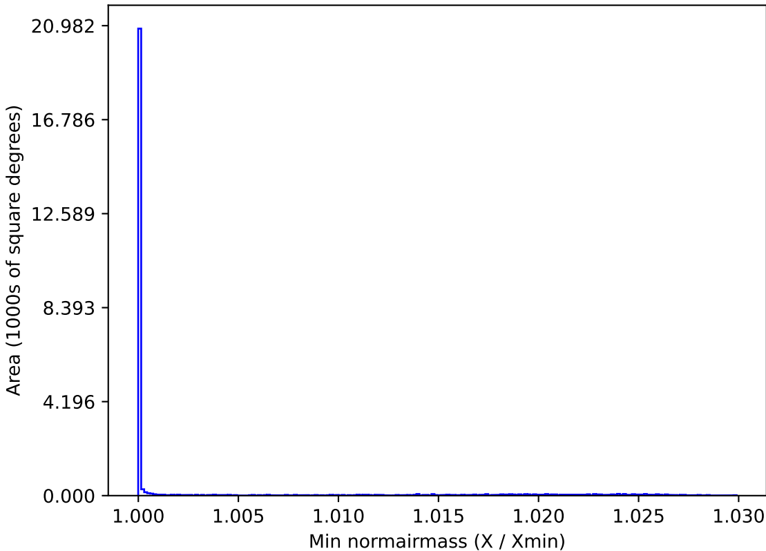
too_elab_r16_d2_griz_v3.4_10yrs All sky all bands: Min normairmass
