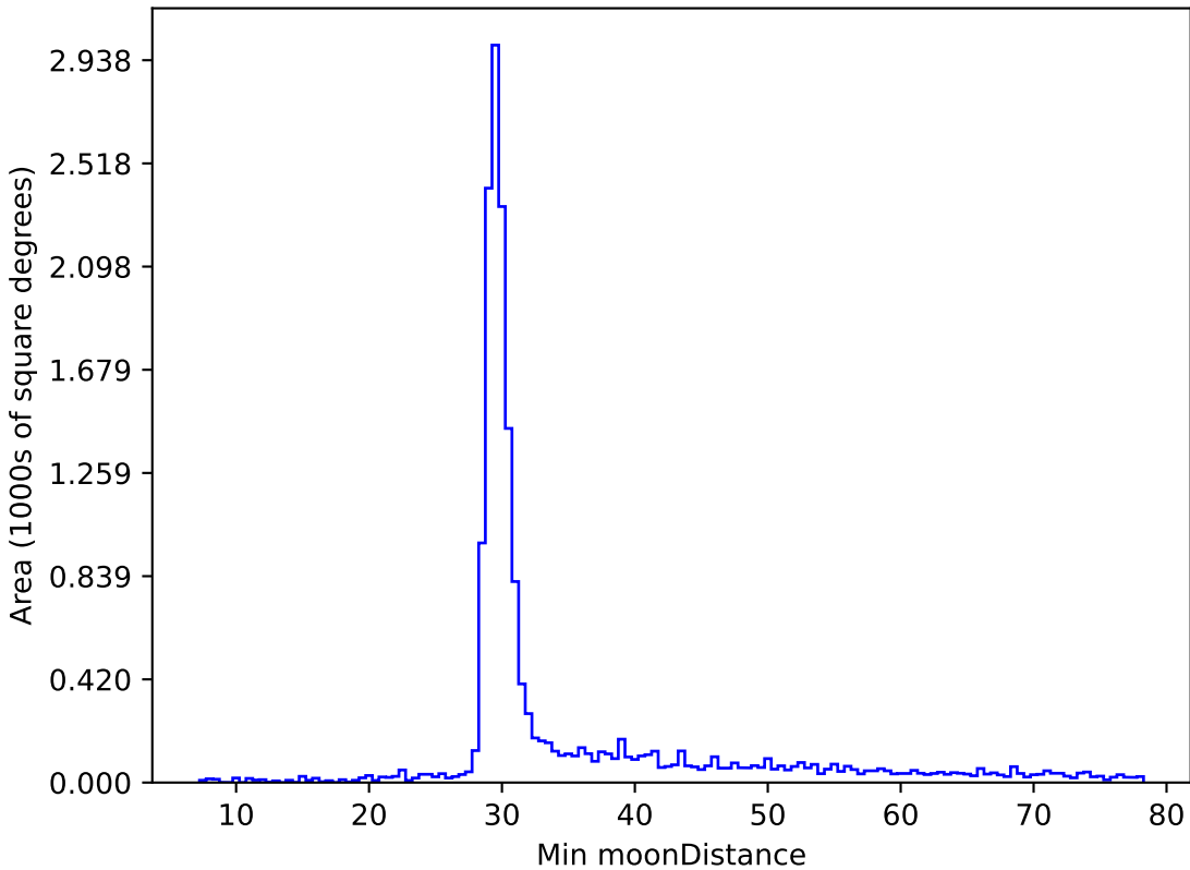
too_elab_r16_d2_griz_v3.4_10yrs WFD z band: Min moonDistance
