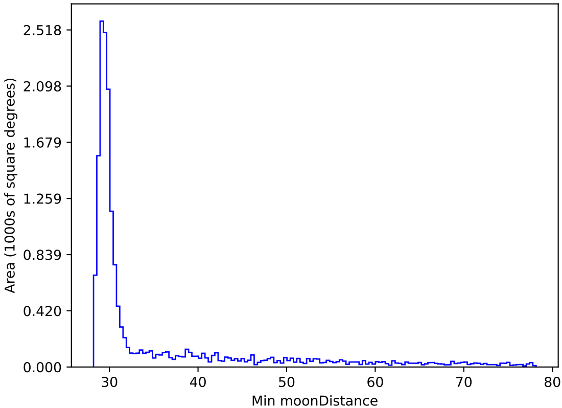
too_elab_r16_d2_griz_v3.4_10yrs WFD y band: Min moonDistance
