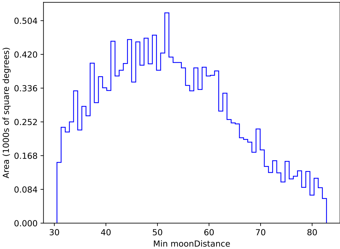
too_elab_r16_d2_griz_v3.4_10yrs WFD u band: Min moonDistance
