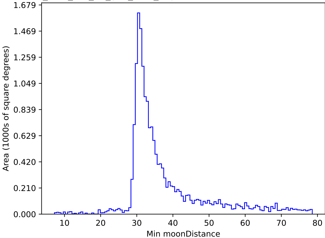
too_elab_r16_d2_griz_v3.4_10yrs WFD r band: Min moonDistance
