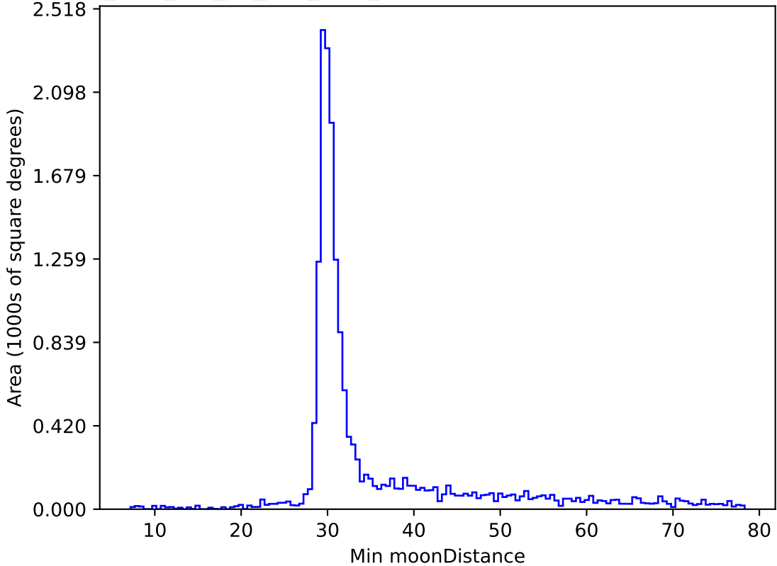
too_elab_r16_d2_griz_v3.4_10yrs WFD i band: Min moonDistance
