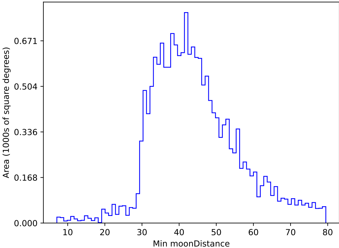
too_elab_r16_d2_griz_v3.4_10yrs WFD g band: Min moonDistance
