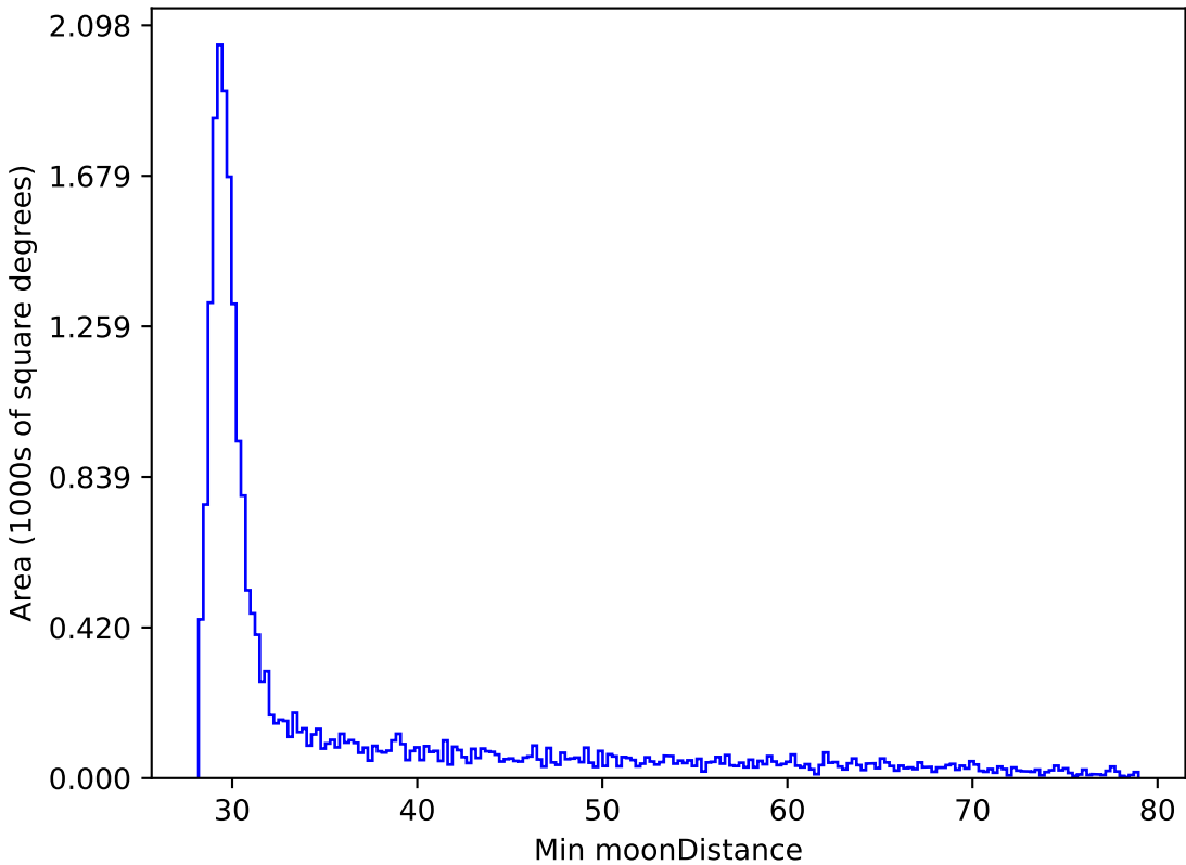
too_elab_r16_d2_griz_v3.4_10yrs All sky y band: Min moonDistance
