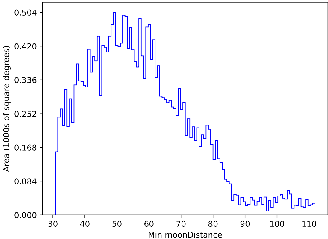
too_elab_r16_d2_griz_v3.4_10yrs All sky u band: Min moonDistance
