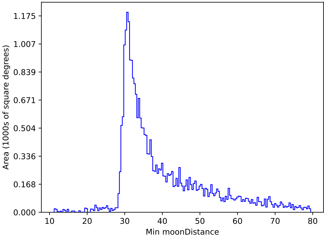
too_elab_r16_d2_griz_v3.4_10yrs All sky r band: Min moonDistance
