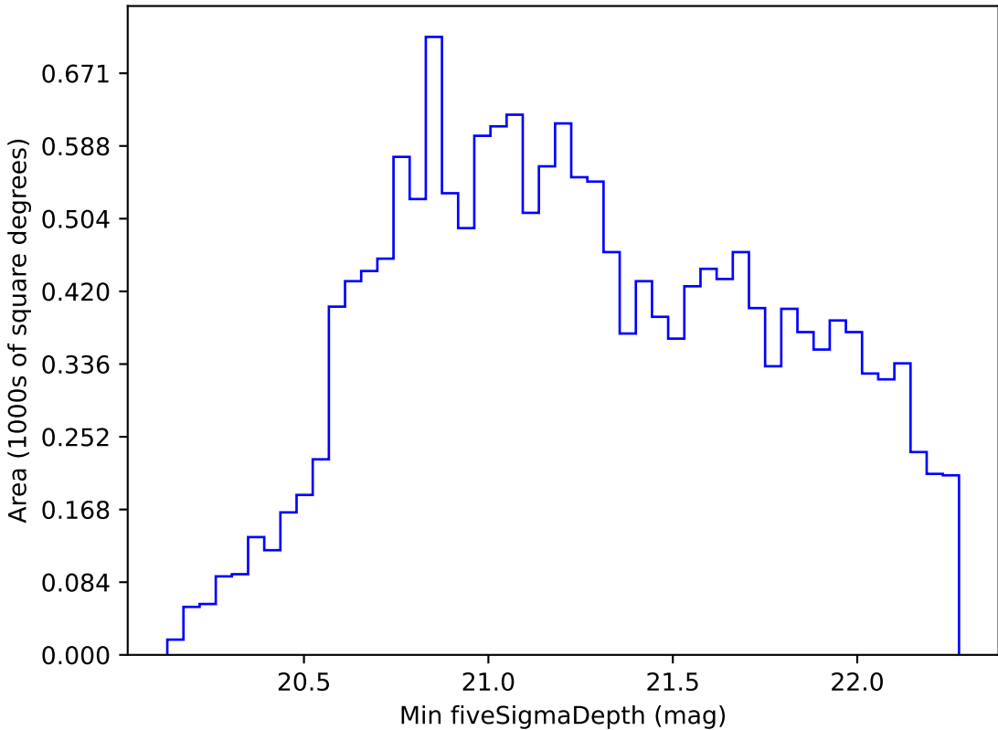
too_elab_r16_d2_griz_v3.4_10yrs WFD z band: Min fiveSigmaDepth
