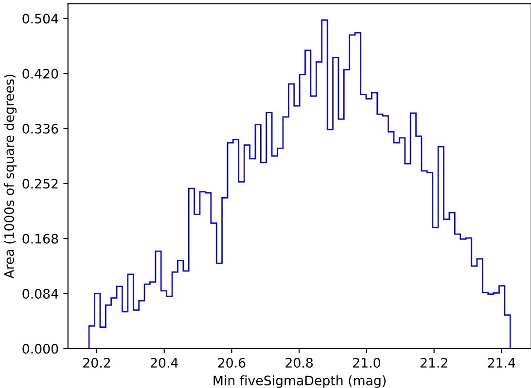
too_elab_r16_d2_griz_v3.4_10yrs WFD y band: Min fiveSigmaDepth
