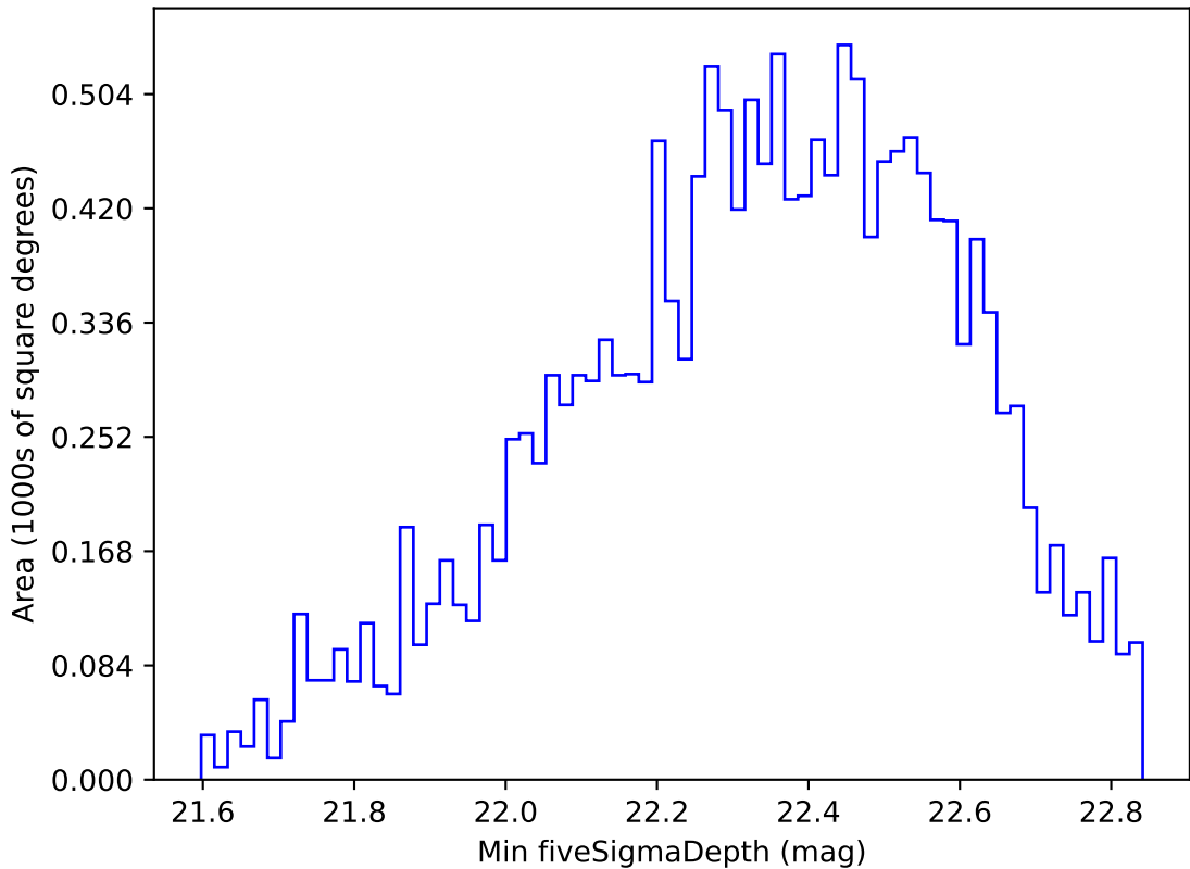
too_elab_r16_d2_griz_v3.4_10yrs WFD u band: Min fiveSigmaDepth
