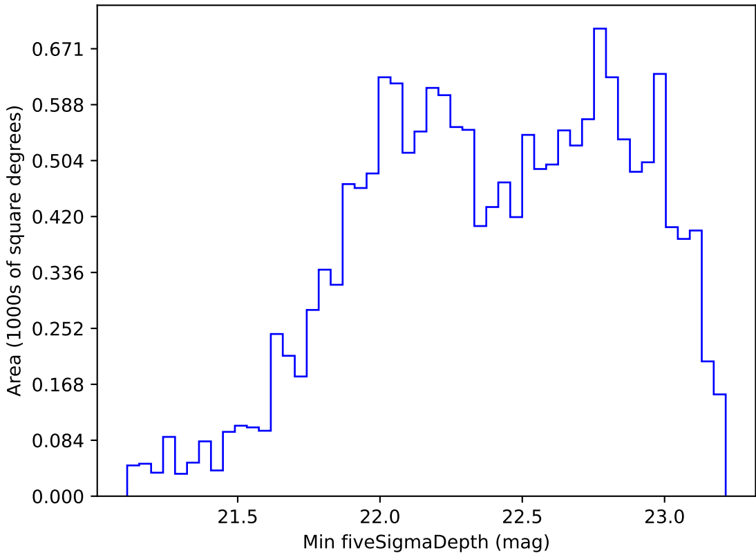
too_elab_r16_d2_griz_v3.4_10yrs WFD r band: Min fiveSigmaDepth
